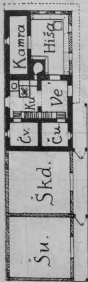
1. Znoter dvor Jereka, Bohinj XVIII. st.
